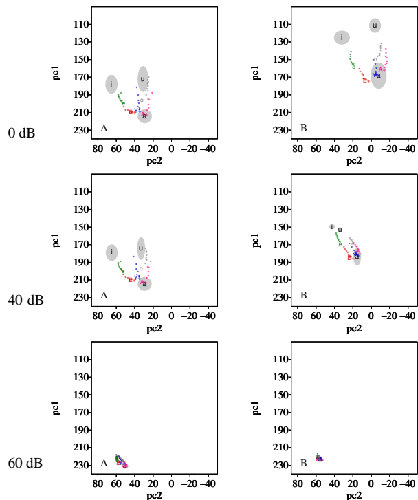
Figure 2: Speaker A (rather poor recording quality) and speaker B (good recording quality) before (top) and after (bottom) increasing filter minimum values. Increasing the minimal filter values results in decreasing sizes and shifting positions of the vowel space. One sigma ellipses represent /a/, /i/, /u/. The points indicate 10ms steps in time of the mean vowel movement for /o:/, /e:/, /ɛɪ/, /ʌy/ and /au/.
