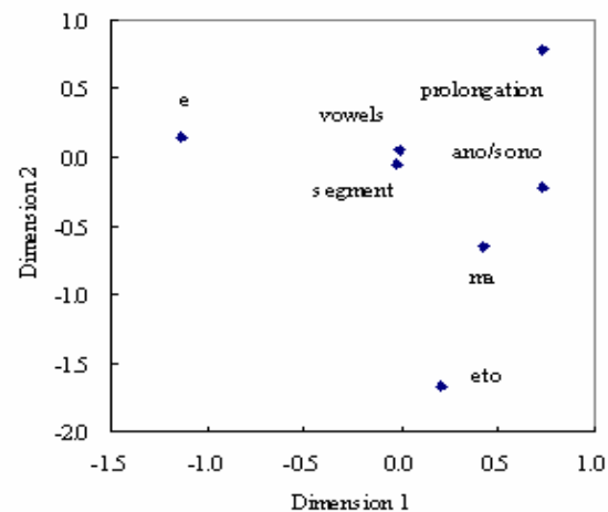
Figure 1: A symmetric map of the first two dimensions for filler types. The first dimension separates e from other types and the second dimension set apart eto and prolongations in opposite directions from other fillers.
