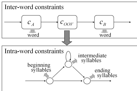
Fig. 1. A hierarchical language model
