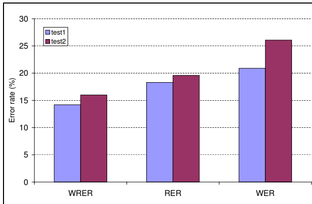
Figure 4: Variation of WRR, RER and WER with two different test corpus.
