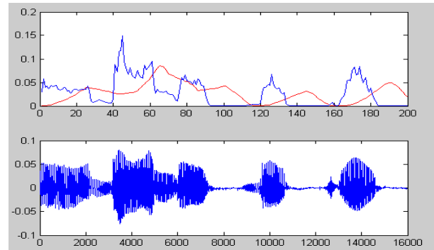
Fig.2. Entropy compared to its moving average.
