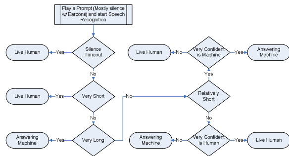
Figure 2: Call Classifier using both utterance length and recognized text
