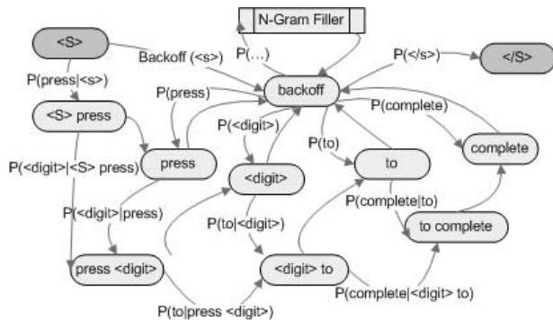
Figure 1: Interpolated N-gram Model. (Transitions w/o labels are back-off transitions)
