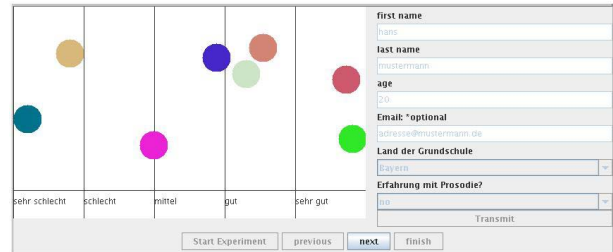
Figure 2. Java interface for subjective evaluation. Subjects should position stimuli by drag and drop (the natural utterance + synthetic renderings by 7 different prosodic models) on a MOS scale. Subjects can listen to stimuli as much as required (simple-click) for taking their decision.
