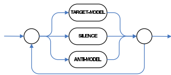
Figure 2: Simple Network of Digit Detector.
