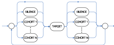
Figure 3: General Network of Digit Detector.
