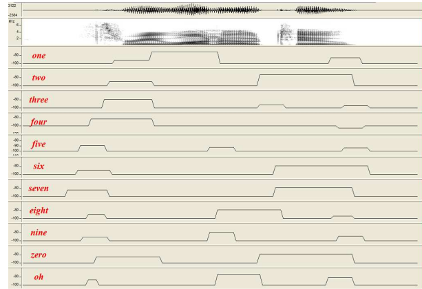
Figure 4: Hypotheses Generated by 11 Detectors.
