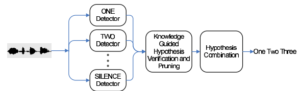
Figure 1: Framework of Detection-based ASR System.
