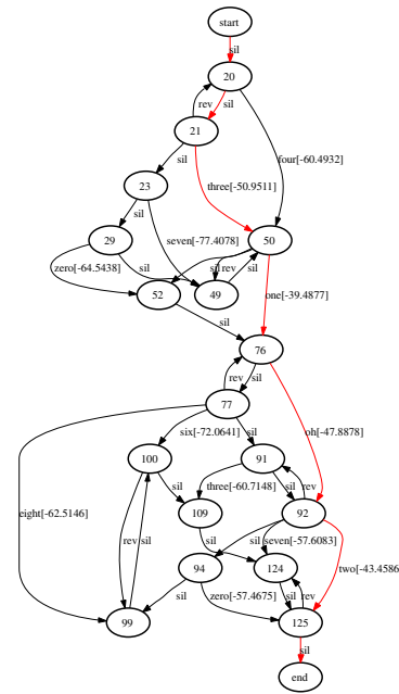
Figure 5: Weighted Directed Graph.
